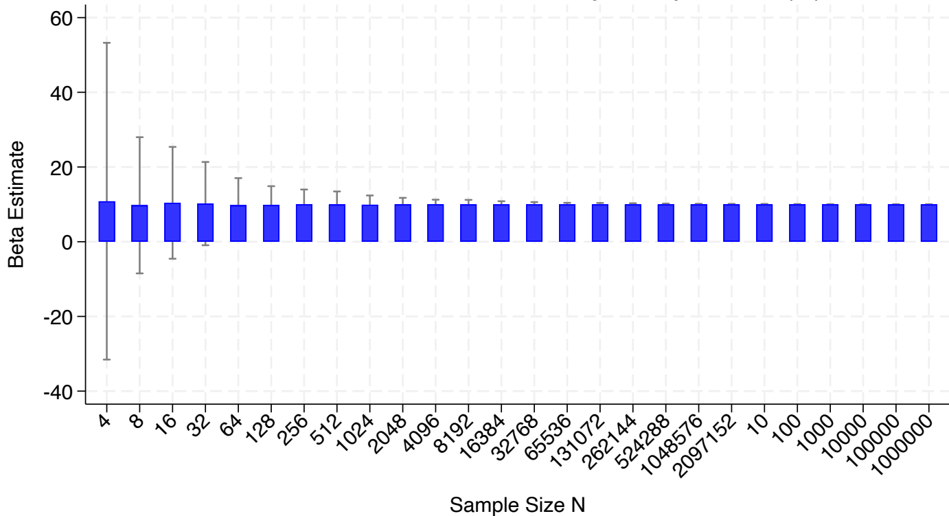
Beta Estimates with 95% CI by Sample Size (N)
